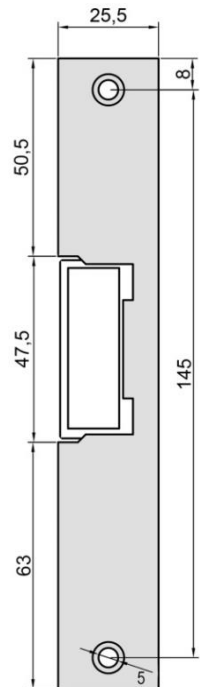
Mortice Faceplate dimensions
